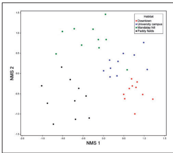
Figure 4. NMS ordination of sampling locations color-coded by habitat types. The first and second NMS axes represent 43% and 32% of the variance.
